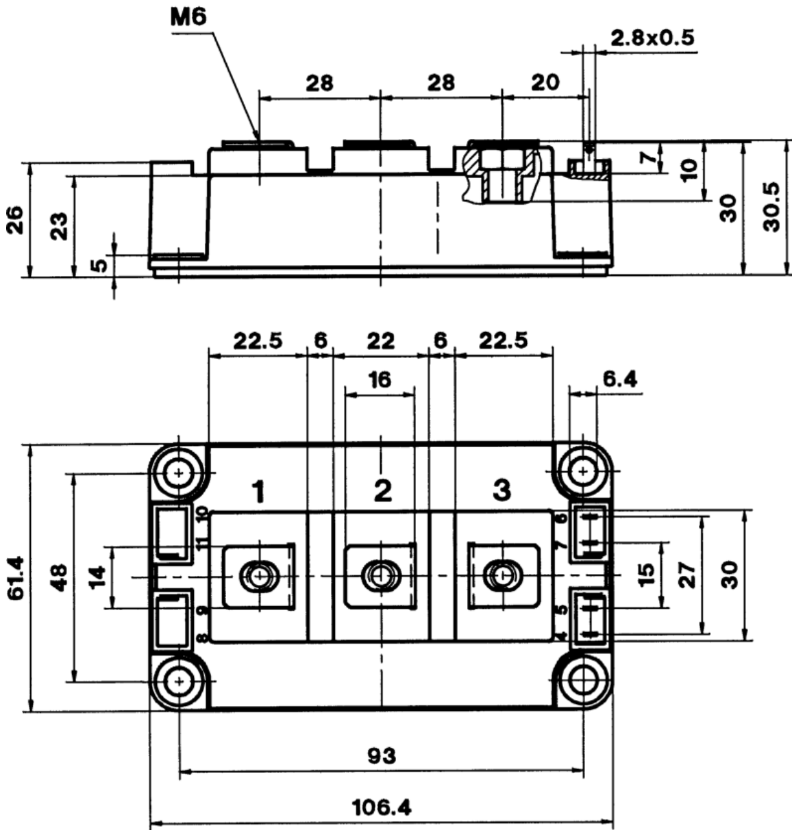
SEMITRANS 3
